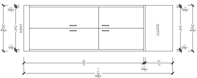
D ELEVATION
