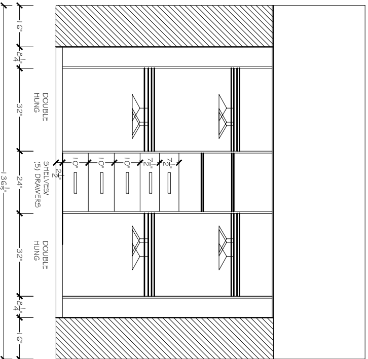
C ELEVATION
